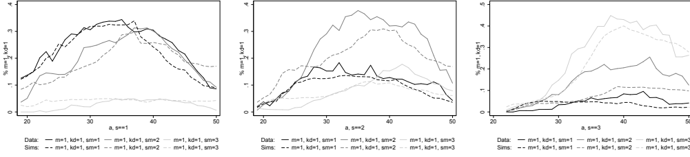
Figure 5: Fit of key lifecycle moments
